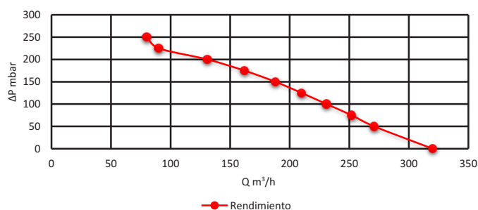
TKW3 EX 3 kW
